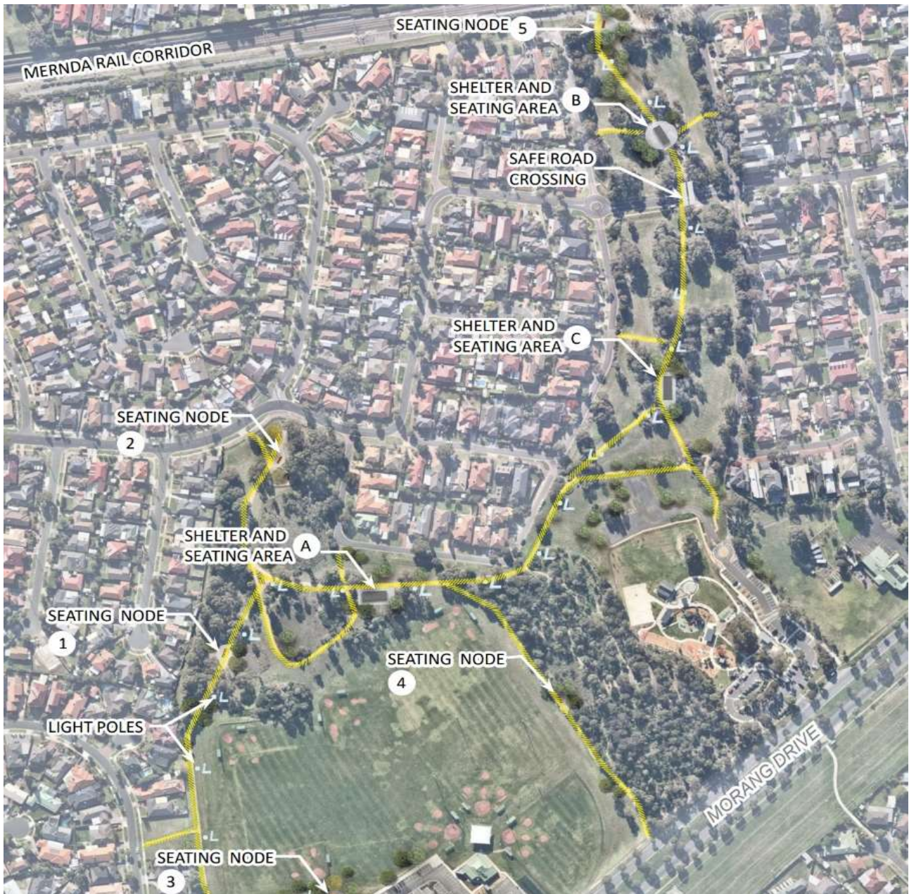
Figure 1- Site Plan
